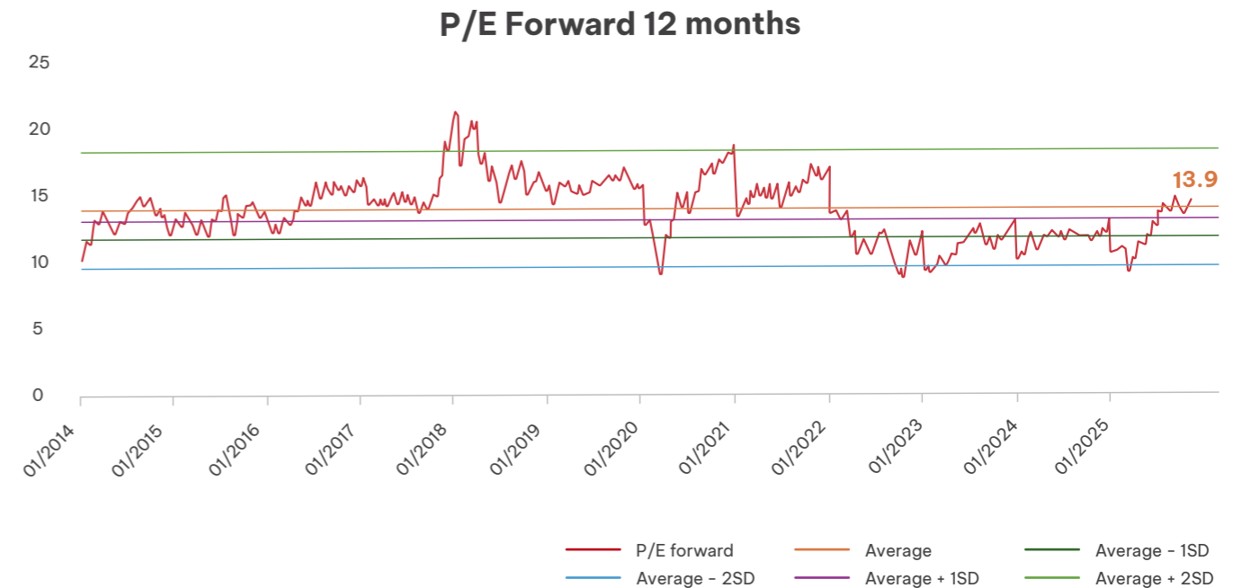
Figure 29: 10-year P/E of VN-INDEX
